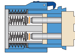
Enclosed arc chambers keep arcs safely contained
